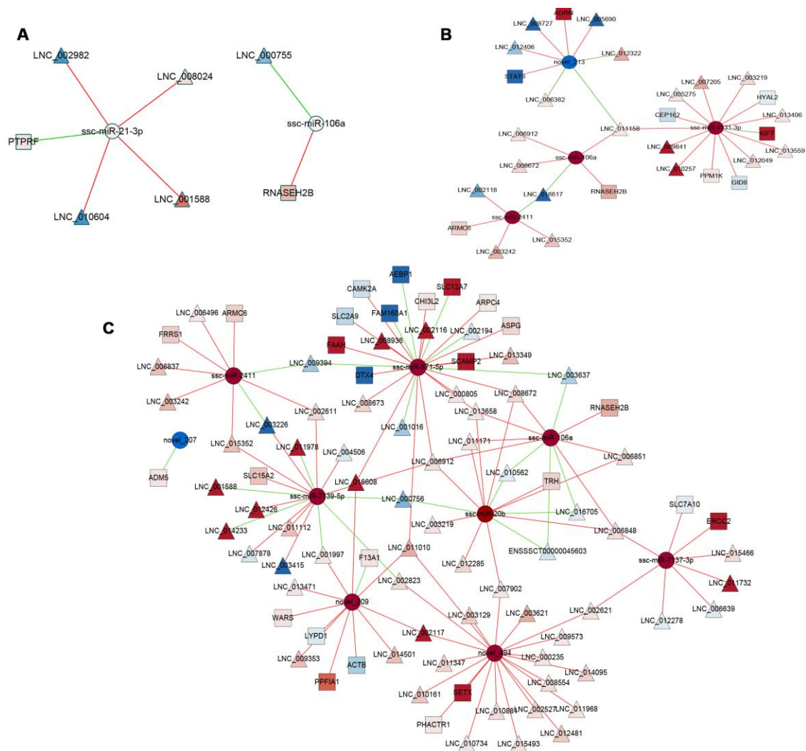
19 Figure S4: Regulatory network of lncRNAs and mRNA-miRNAs of HPS (A), PRRSV (B), and PRRSV-HPS (C) 20 groups. The rectangles indicate mRNAs, the triangles represent lncRNAs, and the circles indicate miRNAs. A 21 gradient from green to red represents downregulated to upregulated, respectively.
