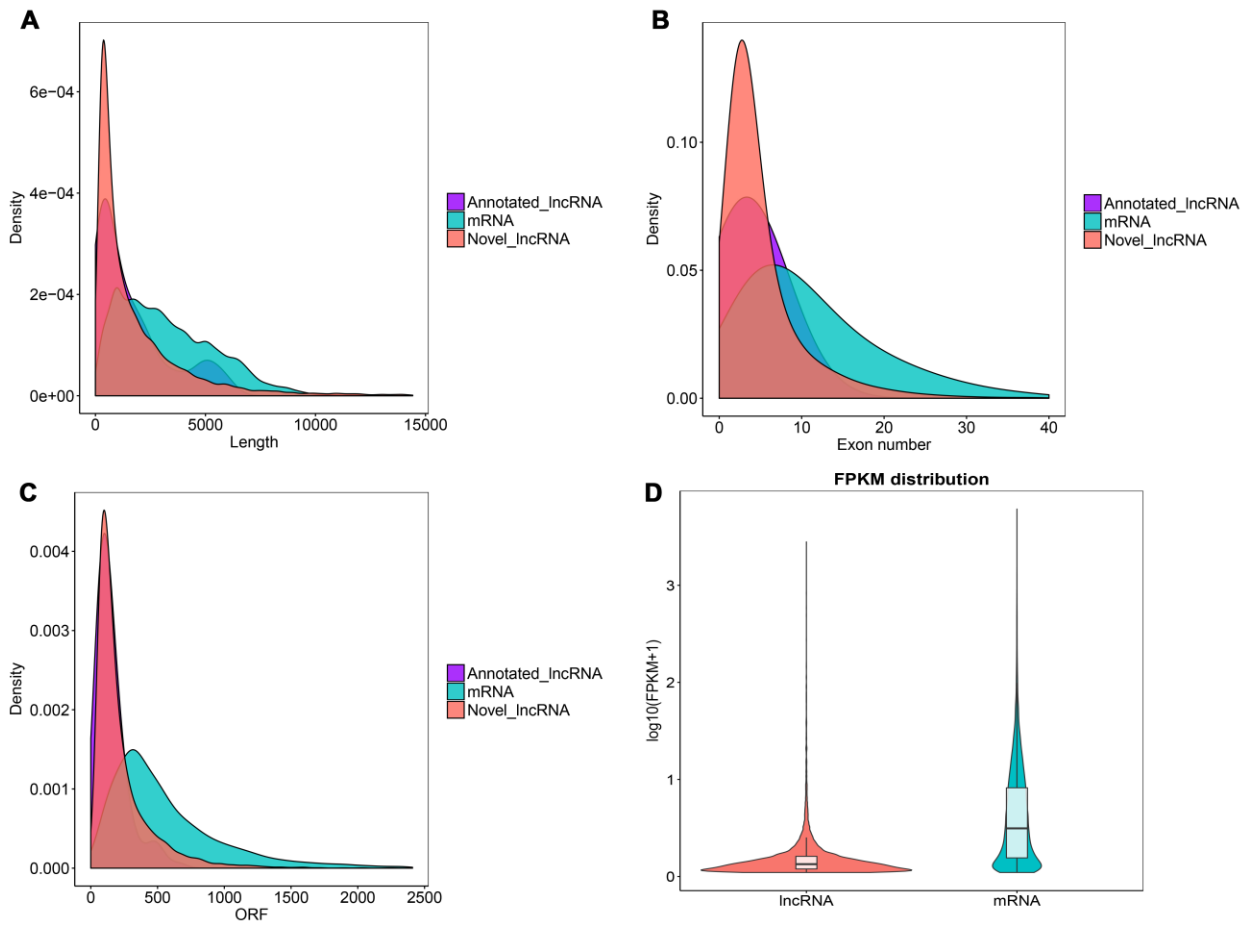
4 Figure S1: The characteristics of lncRNAs.
