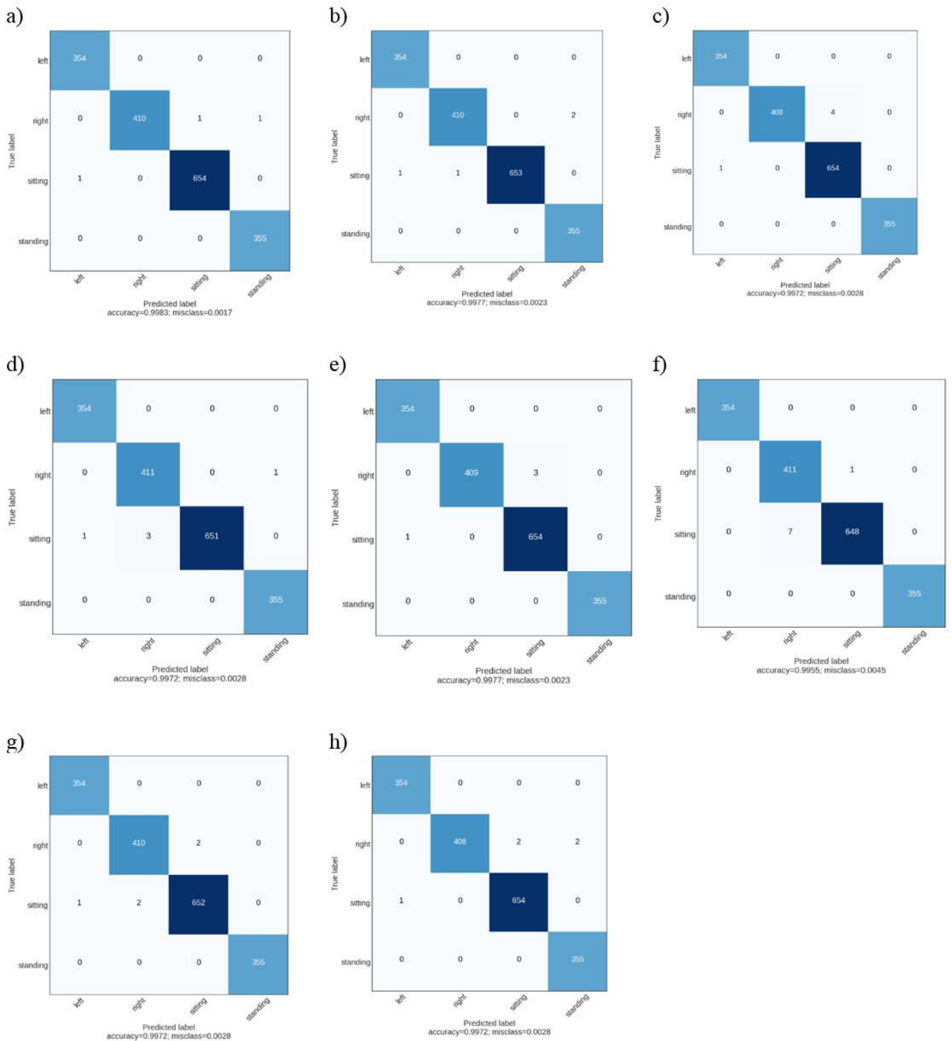
Figure 3. Confusion matrix of swine behavior image classification: a) DenseNet121, b) DenseNet201, c) InceptionResNetV2, d) InceptionV3, e) MobileNet, f) VGG16, g) VGG19, and h) Xception.
