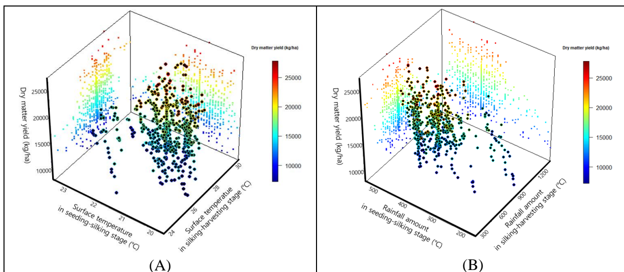
1 Figure 3. Scatter plots for seasonal effect of soil surface temperature and rainfall amount between before 2 and after silking stage: (A) soil surface temperature, (B) rainfall amount
