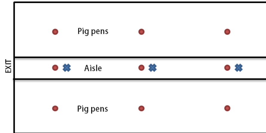
Figure 2 Sampling points for the environmental parameters. ● Sampling points for temperature, relative humidity, and air speed. ✖ Sampling points for concentration of particulate matter, airborne bacterial, and gases (CO 2 , NH 3 , H 2 S).
