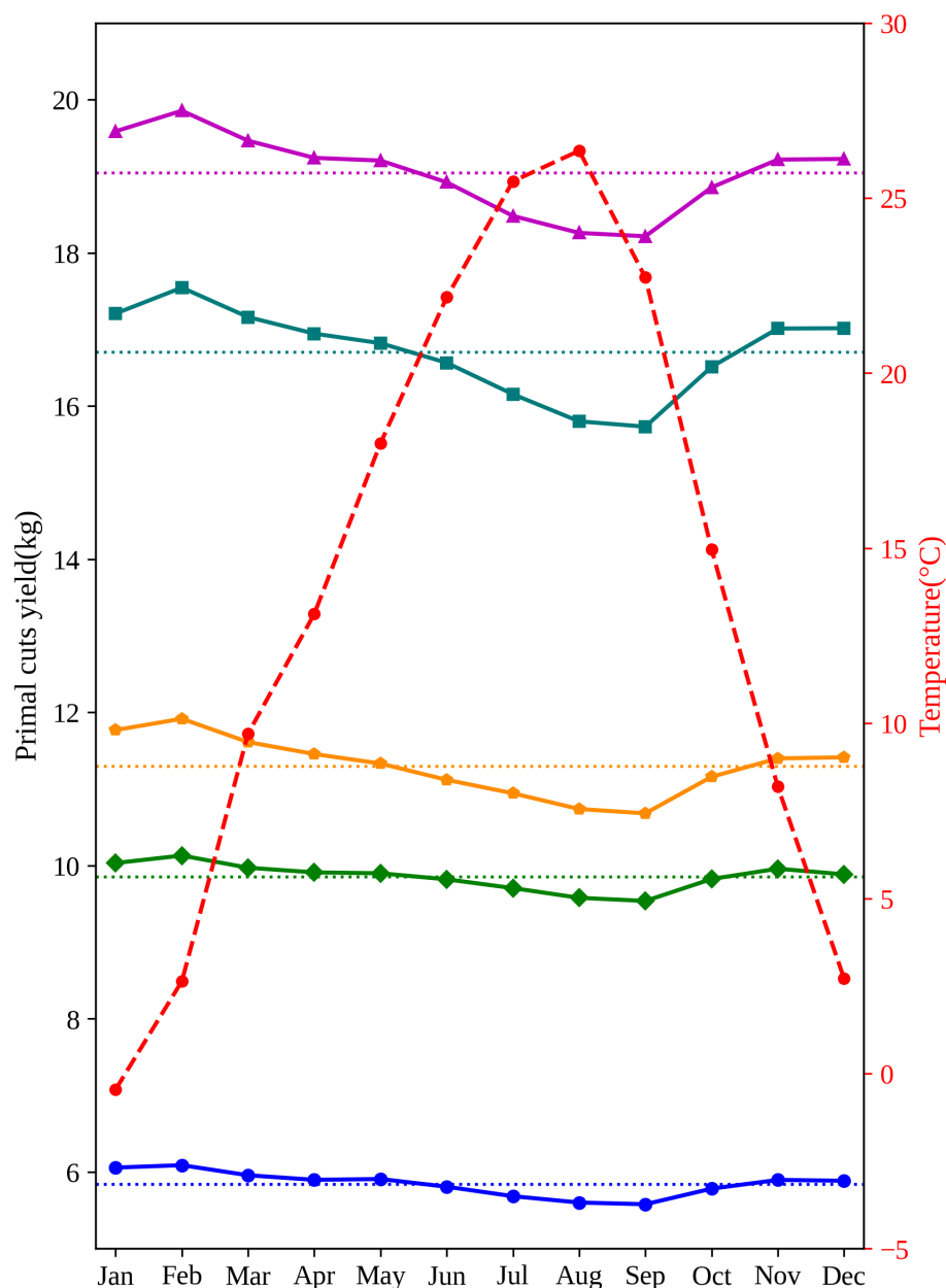
Fig. 2. Monthly production of LYD pork primal cuts as affected by temperature in 2023. Monthly sample number: Jan, 58,011 pigs; Feb, 60,702 pigs; Mar, 67,156 pigs; Apr, 55,607 pigs; May, 63,600 pigs; Jun, 54,292 pigs; Jul, 50,058 pigs; Aug, 57,627 pigs; Sep, 50,134 pigs; Oct, 62,688 pigs; Nov, 63,325 pigs; Dec, 56,527 pigs. Each graph, from top to bottom, represents ham (solid line with triangles), belly (solid line with squares), shoulder picnic (solid line with pentagons), loin (solid line with diamonds), and shoulder blade (solid line with circles). The dotted line represents the average (dotted line) of each primal cut, and the red dotted line indicates the temperature (dotted line with circles).
