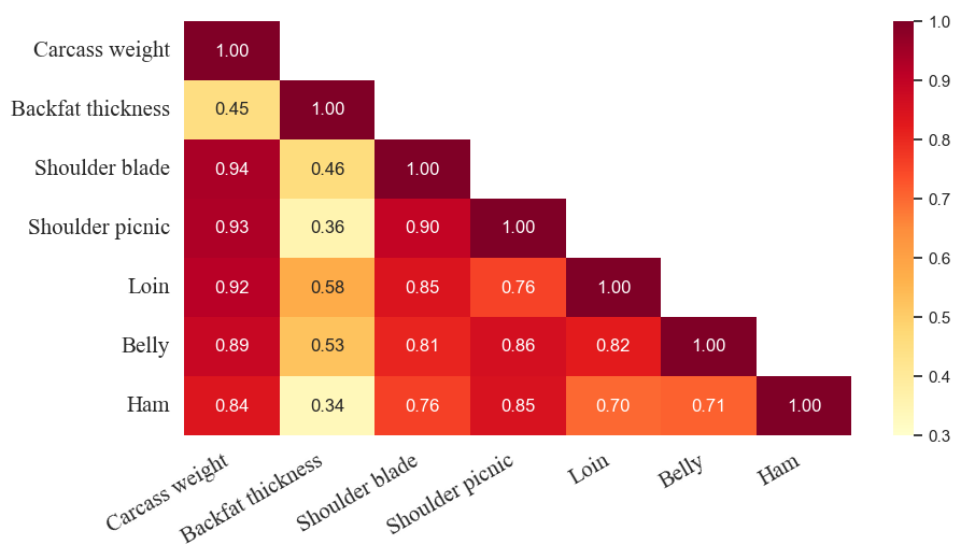
Fig. 1. Heatmap of Pearson correlations among carcass weight, backfat thickness, and primal cuts in LYD pigs. Sample number was 699,727 pigs. All correlations are statistically significant ( p < 0.001 ).
